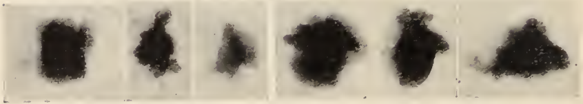
Colonies few.
